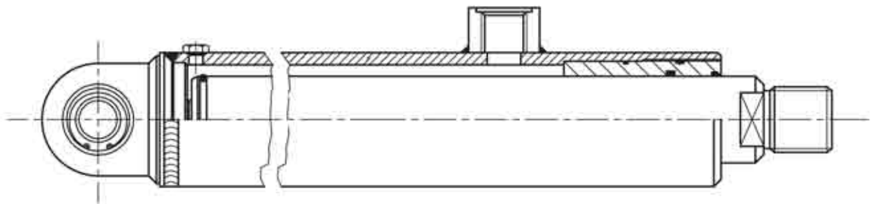
CYLINDER FOR PRESSURE OF 160 bar (TYPE P1B)
